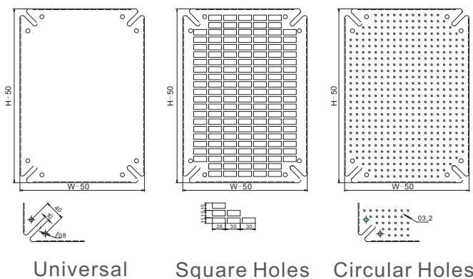
Mounting plate for wall mount enclosure
