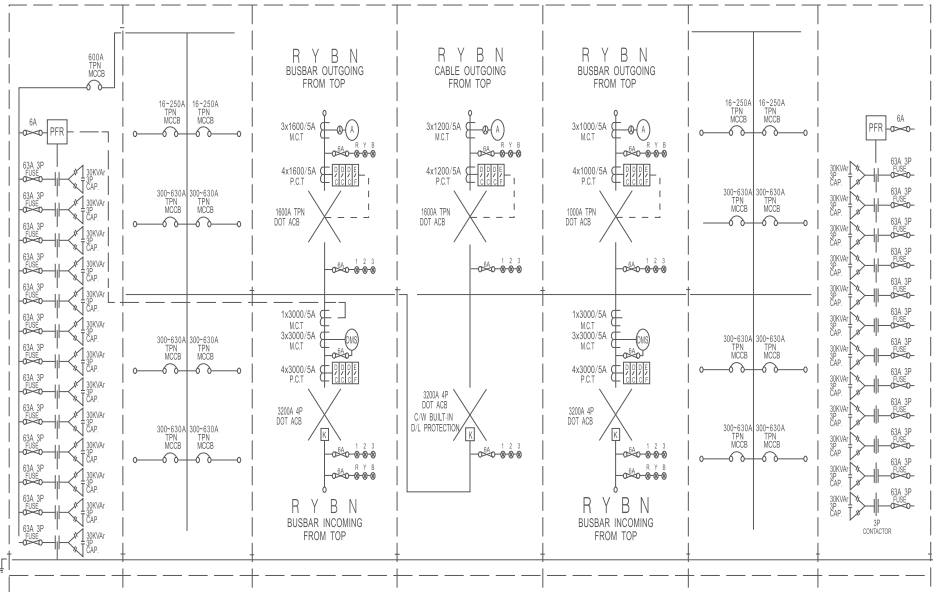
SINGLE LINE BUSBAR DIAGRAM
