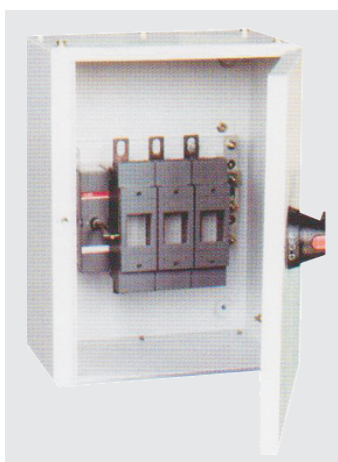
Switch Board with Fuse
